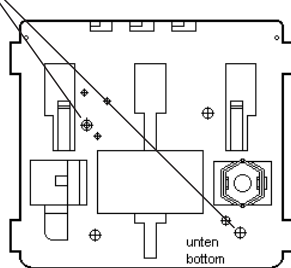
Apparatus mounting plate for pipe mounting
