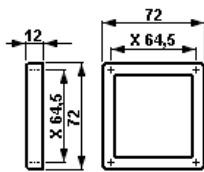
Glass for measuring instrument AM/VM72
